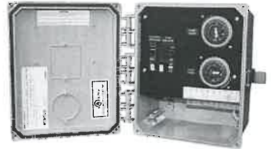
C-85 & C-95, 240V, Single Phase Control Panel for 240V Kasco Fountain, Aerator, and/or Circulator Models
